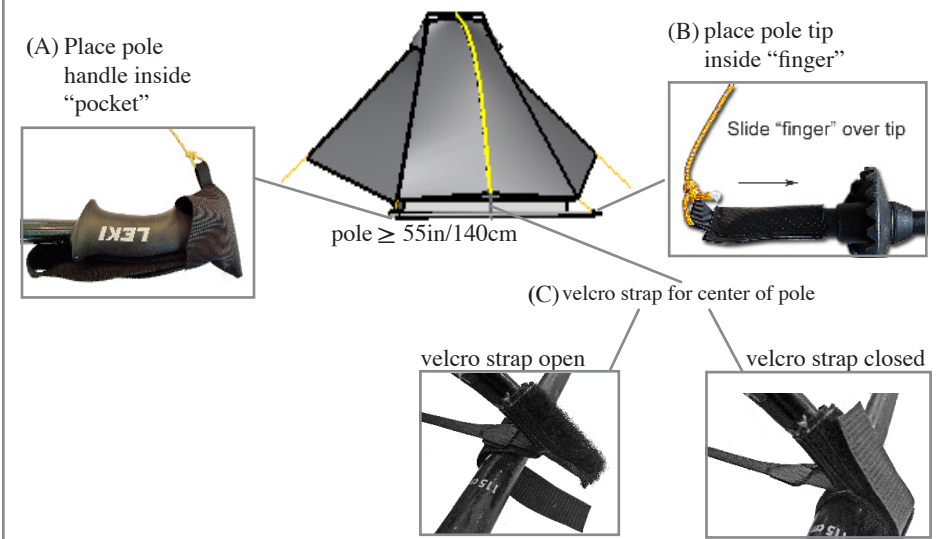
Image 3: Free standing set-up
